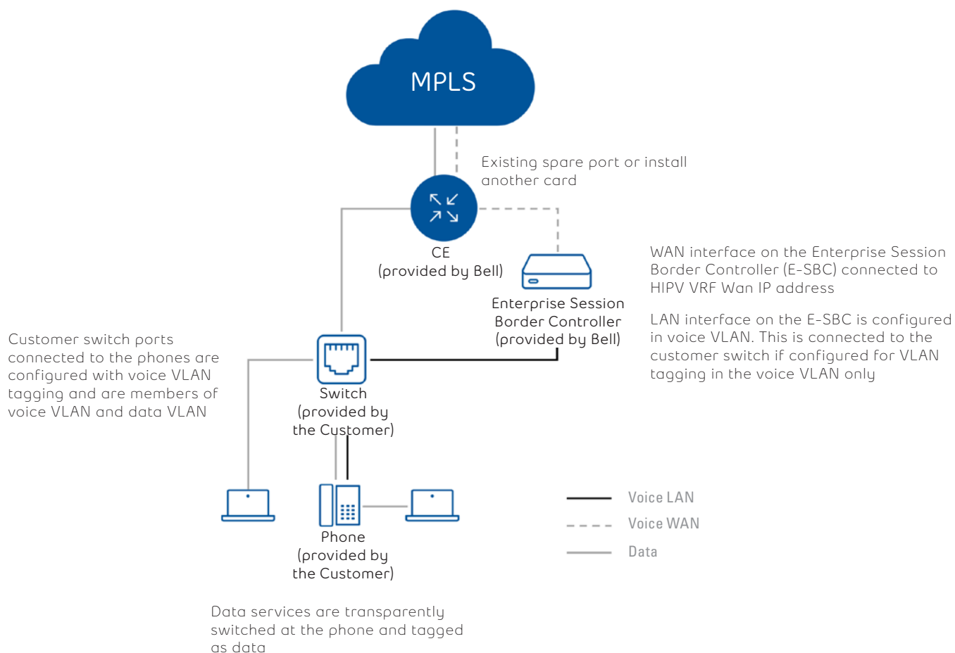
Figure 1. Basic LAN architecture
